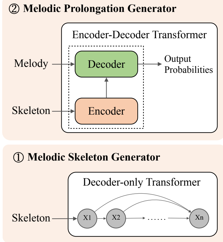
(b) Overall Architecture of WuYun
