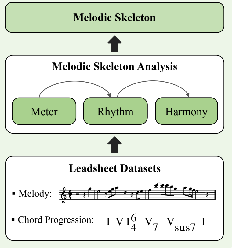
(a) Melodic Skeleton Extraction
