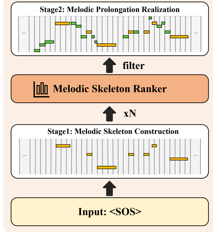
(c) Two-Stage Melody Generation
